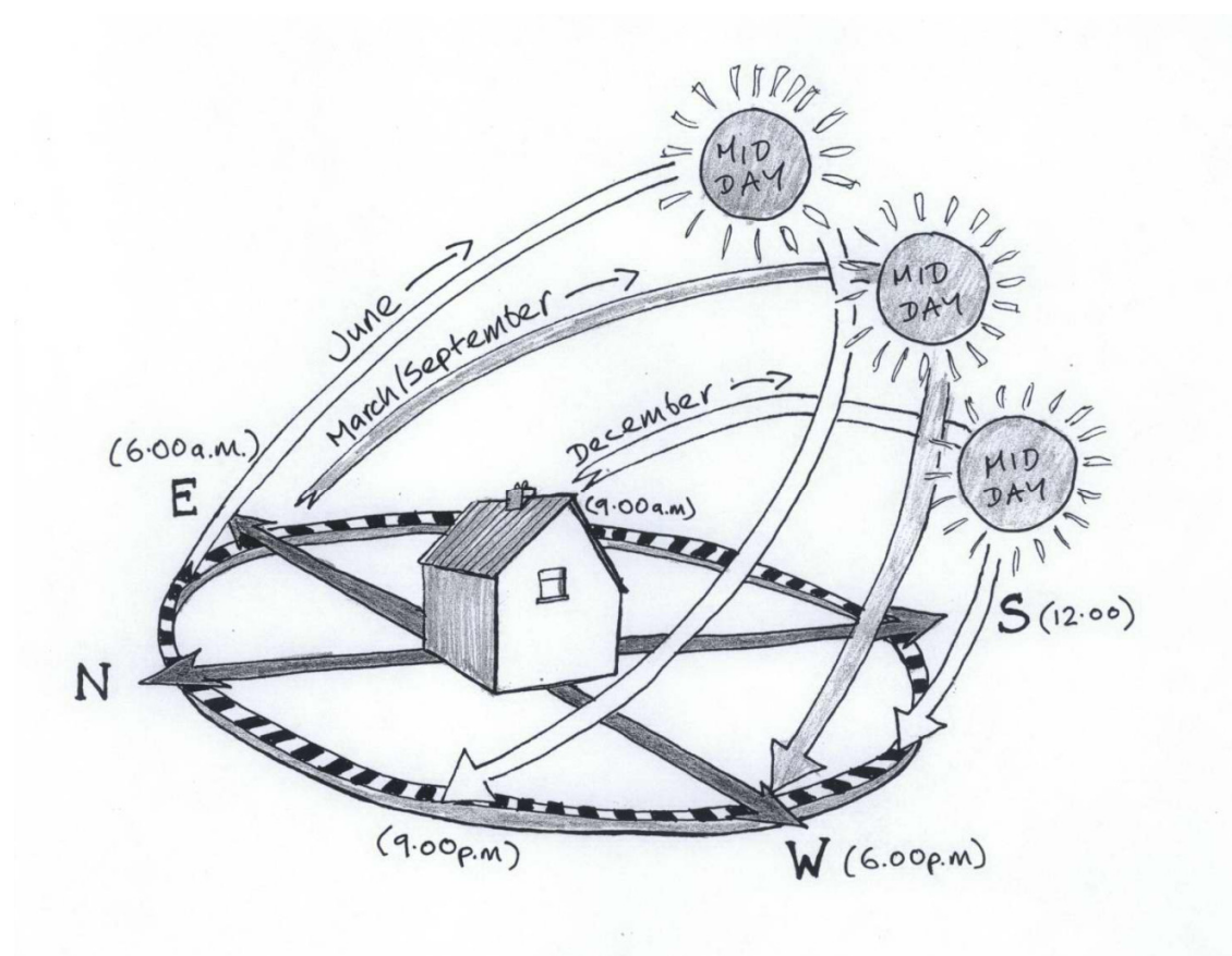
Diagram 2 – sun path
